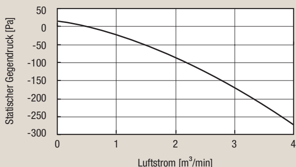
PCFY-P40VKM-E
